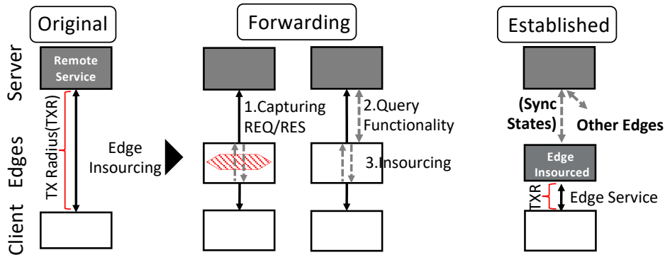
Figure 8: Distributed Architecture for Edge Insourcing
