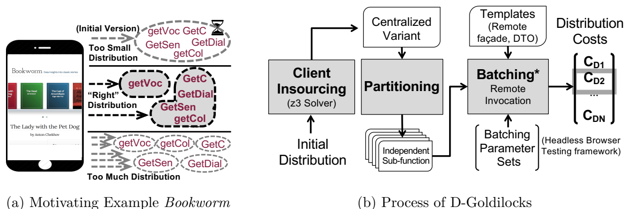
Figure 6: D-Goldilocks for Optimizing Remote Execution Granularity
